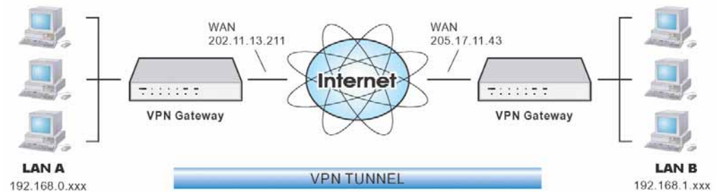
Figure 99: Connecting 2 ADW-4302v2s
